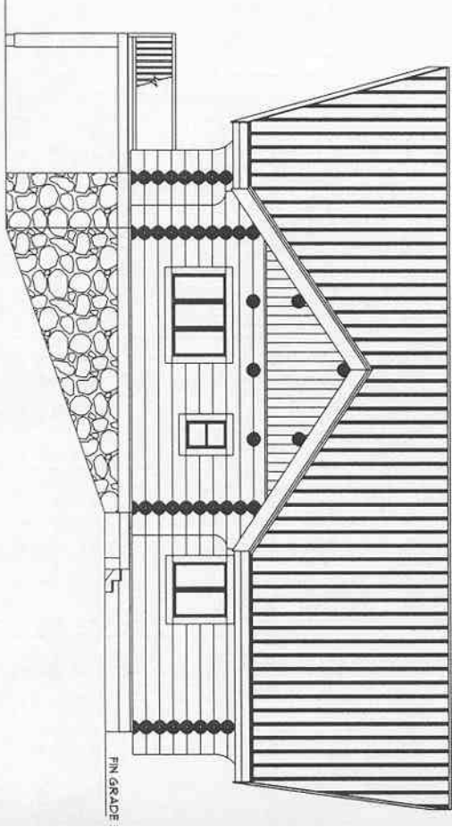
LEFT ELEVATION
